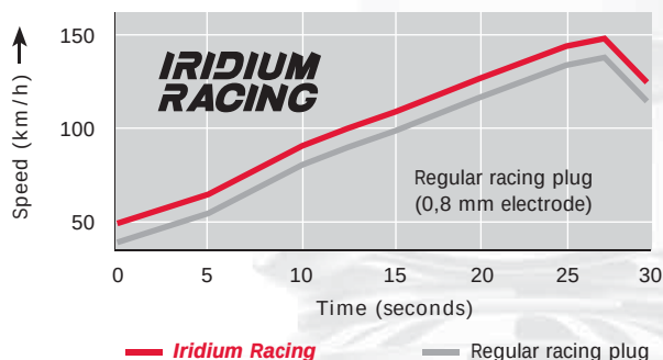
Improved Acceleration Data: In-Company Comparison
